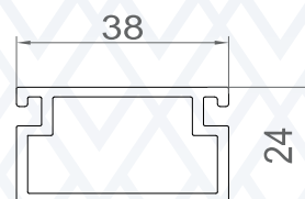
AXL-CN-02 Track Connector
