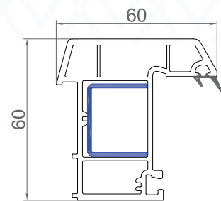
BLC-FM-01 Casement Fly Mullion
