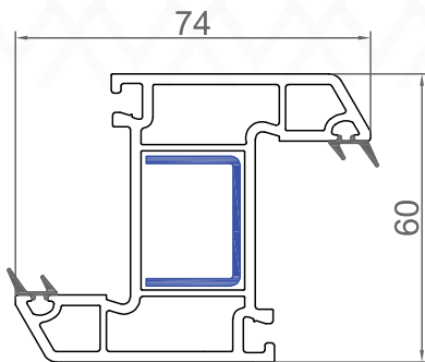
BLC-ZM-01 Z-Mullion Frame Profile
