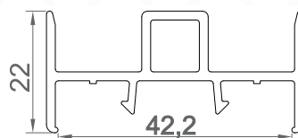
AXL-CN-03 Inline Sash Adoptor
