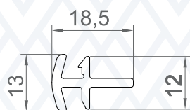
AXL-CP-01 H Coupler
