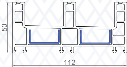
BLS-BF-03 3 Track Outer Frame
