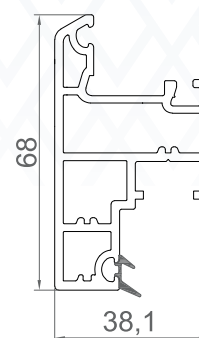
AXL-MF-01 Openable Mesh Frame
