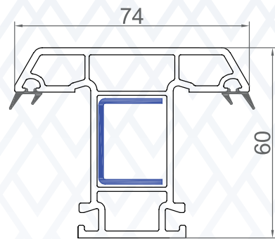
BLC-TM-01 T Mullion
