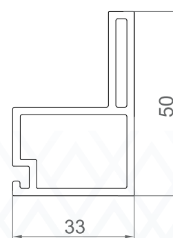
AXL-BF-01 Addon Track
