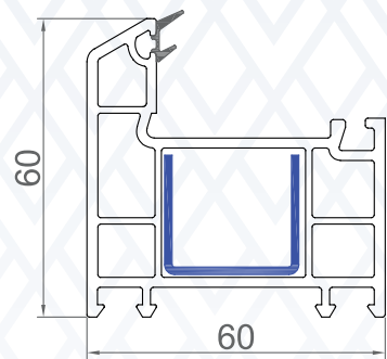
BLC-BF-01 Casement Window Outer Frame
