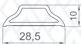
AXL-GB-01 Georgian Bar
