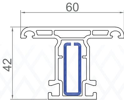
BLS-ML-01 Sash Mullion
