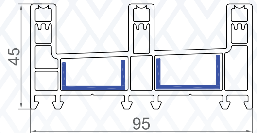
OPS-BF-03 3 Track Outer Frame
