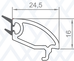
UTL-GB-02 Glazing Bead 24.5 MM
