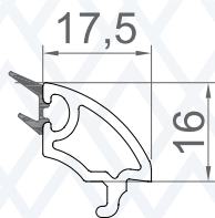
UTL-GB-03 Glazing Bead 17.5 MM
