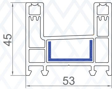
OPS-BF-01 2 Track Outer Frame
